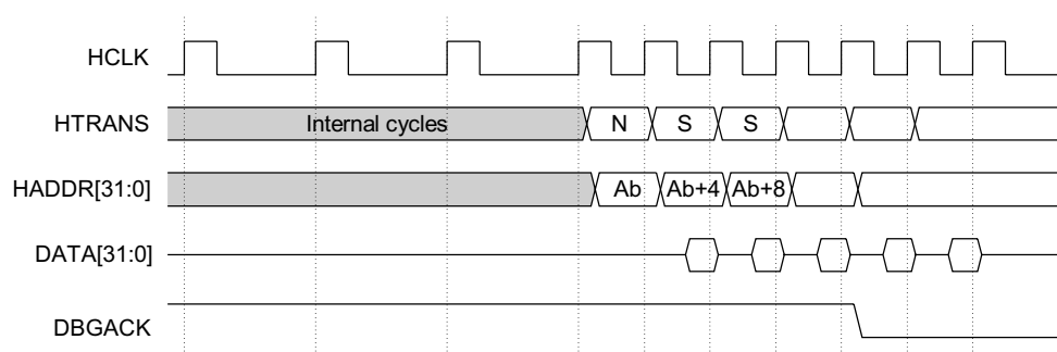
Figure 9-11 Debug exit sequence
